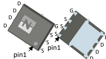
DFN5*6
